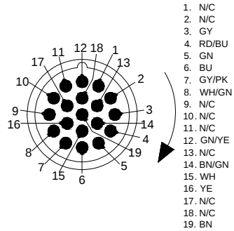
MALE END VIEW
